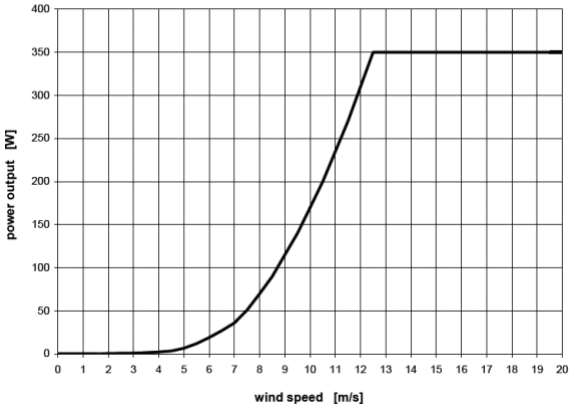
Power Curve
